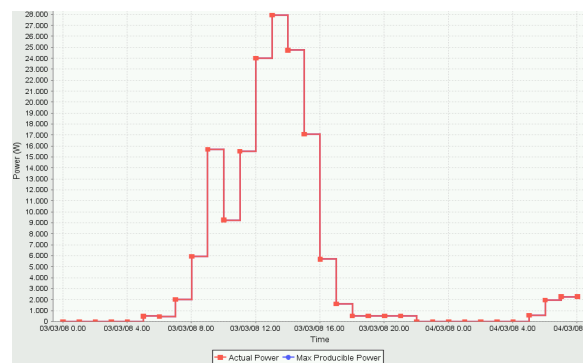
Figure 5. Power produced by photovoltaic plant in the reported experiment
