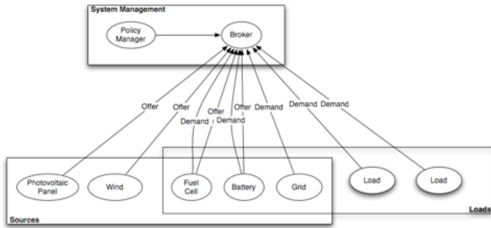
Figure 1. The different agent societies involved in the solution approach
