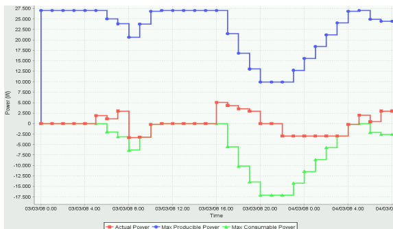
Figure 7. Power supplied by the battery (maximum available power is reported as well)
