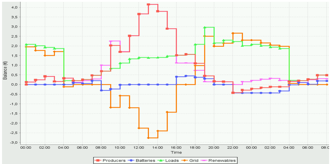
Figure 3. Simulation results for the described case study (power produced/consumed)
