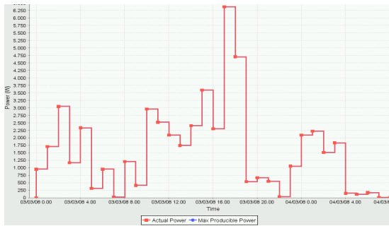
Figure 6. Power produced by wind turbines in the reported experiment
